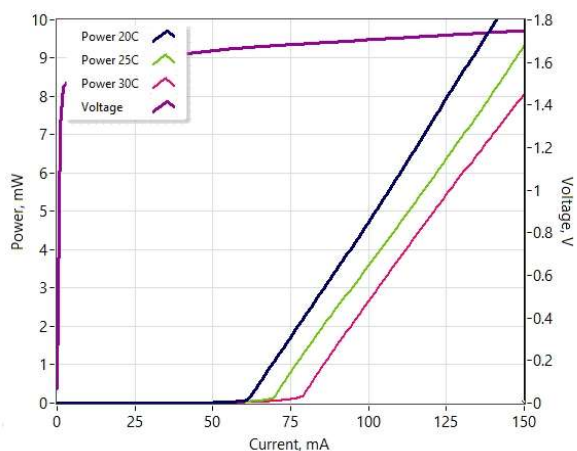
Light Current Voltage Characteristics
