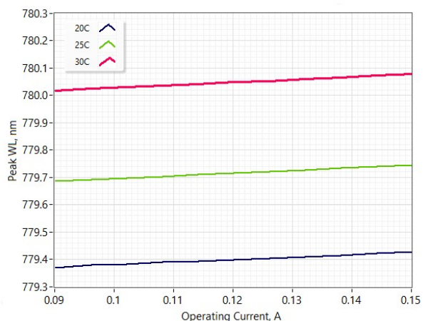
Peak Wavelength Tuning by Current
