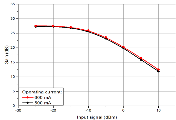
Gain vs. Input signal
