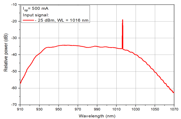
Spectra of amplified optical signal
