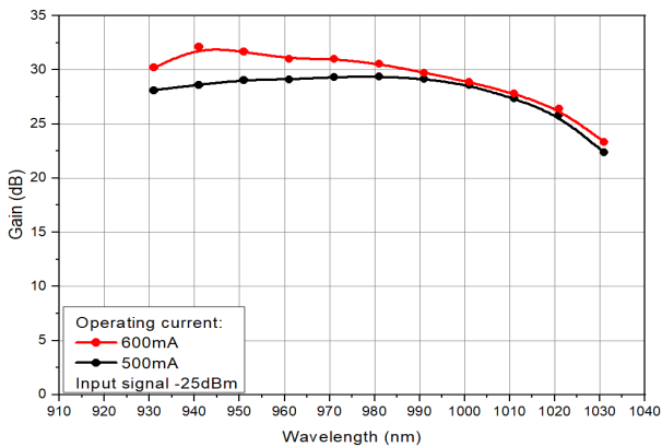
Gain spectra at different currents
