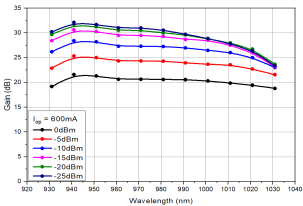
Gain spectra at different input signals
